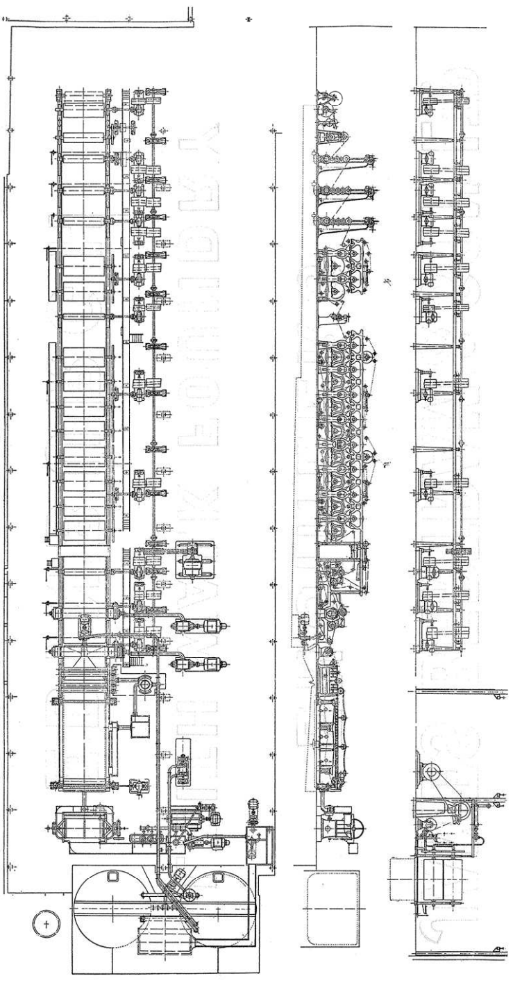
Wire 103 inches wide, 60 feet long, with one 4 feet "Leith Walk" Drum Strainer, Suction Couch, Suction Press, one Plain Press, 20 Drying Cylinders 4 feet diameter, Dry Smoothers, three Calenders, Coolers and Drum Reeler, Enclosed Sectional Worm Driving Gear.
